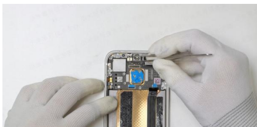
Install the light sensor board into the front case subassembly
