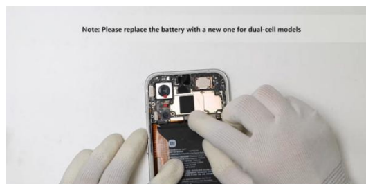
Note: Please replace the battery with a new one for dual-cell models Snap in the BTB cable, and confirm that the cable is not lifted (first snap in battery BTB1, then snap in BTB2)
