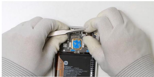
Use tweezers to pry up and remove the earpiece at the disassembly position on the left side of the earpiece; remove the double-sided adhesive tape for earpiece sealing
