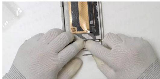
Install the fingerprint module and snap it onto the sub-board fingerprint BTB
