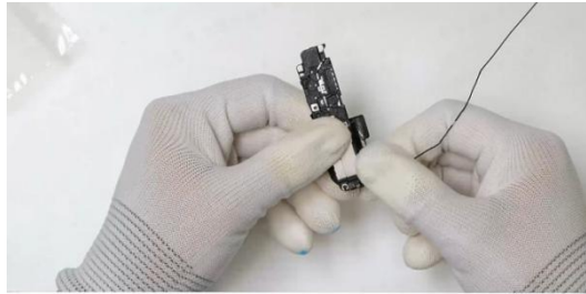
Connect the coaxial cable to the antenna sub-board, route the coaxial cable into the cable slot, and then assemble it to the corresponding position of the lower speaker
