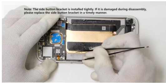
Use tweezers to pry up and remove the side button bracket from the middle frame
