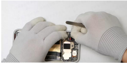
Install the rear main camera and wide-angle camera to the corresponding positions on the mainboard
