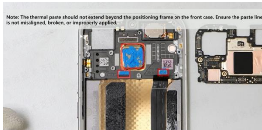
First, use a dispenser to apply thermal paste on the middle frame
