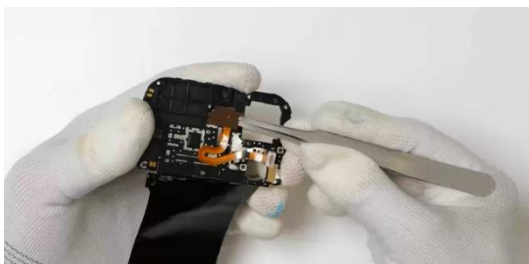
Separate the flashlight FPC assembly from the antenna rear case assembly
