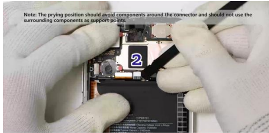
Use anti-static plastic tweezers or pry tools to sequentially disconnect the #2 and #1 battery connectors
