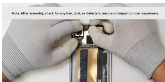
Place the front camera into its position on the front case. Press gently to install it, then secure its connector interface
