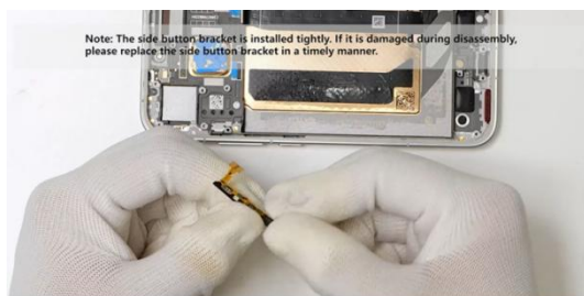
Separate the side button FPC from the side button bracket
